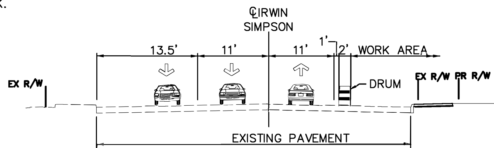
CURB/SIDEWALK CONSTRUCTION NTS
