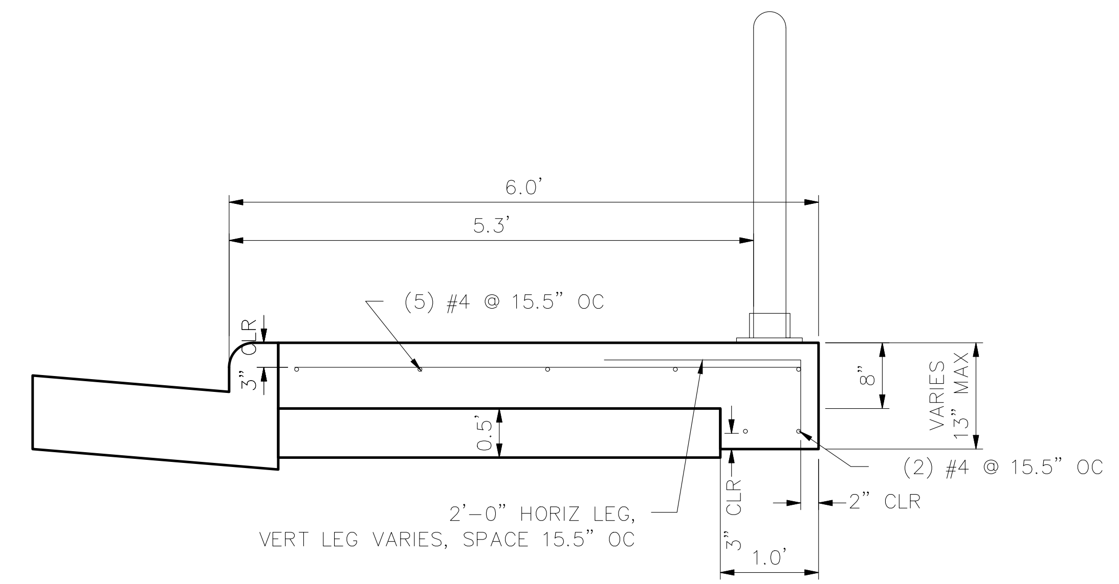
REINFORCED WALK WITH TURNDOWN CURB STA. 50+17.84 TO STA. 50+22.34
