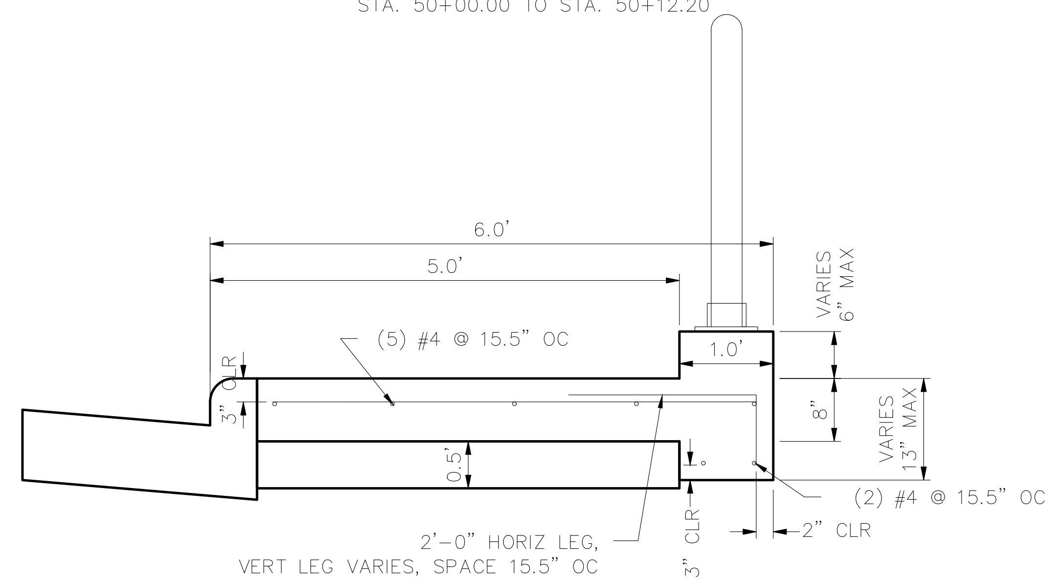
REINFORCED CURB RAMP WITH TURNDOWN CURB STA. 50+12.20 TO STA. 50+17.84
