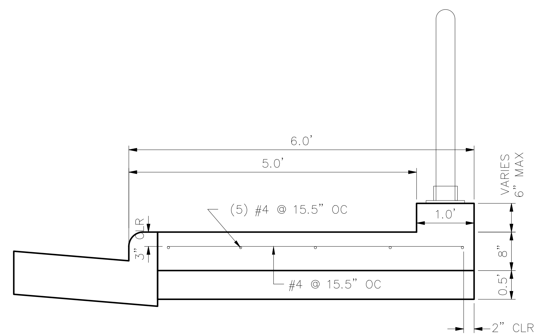
REINFORCED CURB RAMP WITHOUT TURNDOWN CURB STA. 50+00.00 TO STA. 50+12.20
