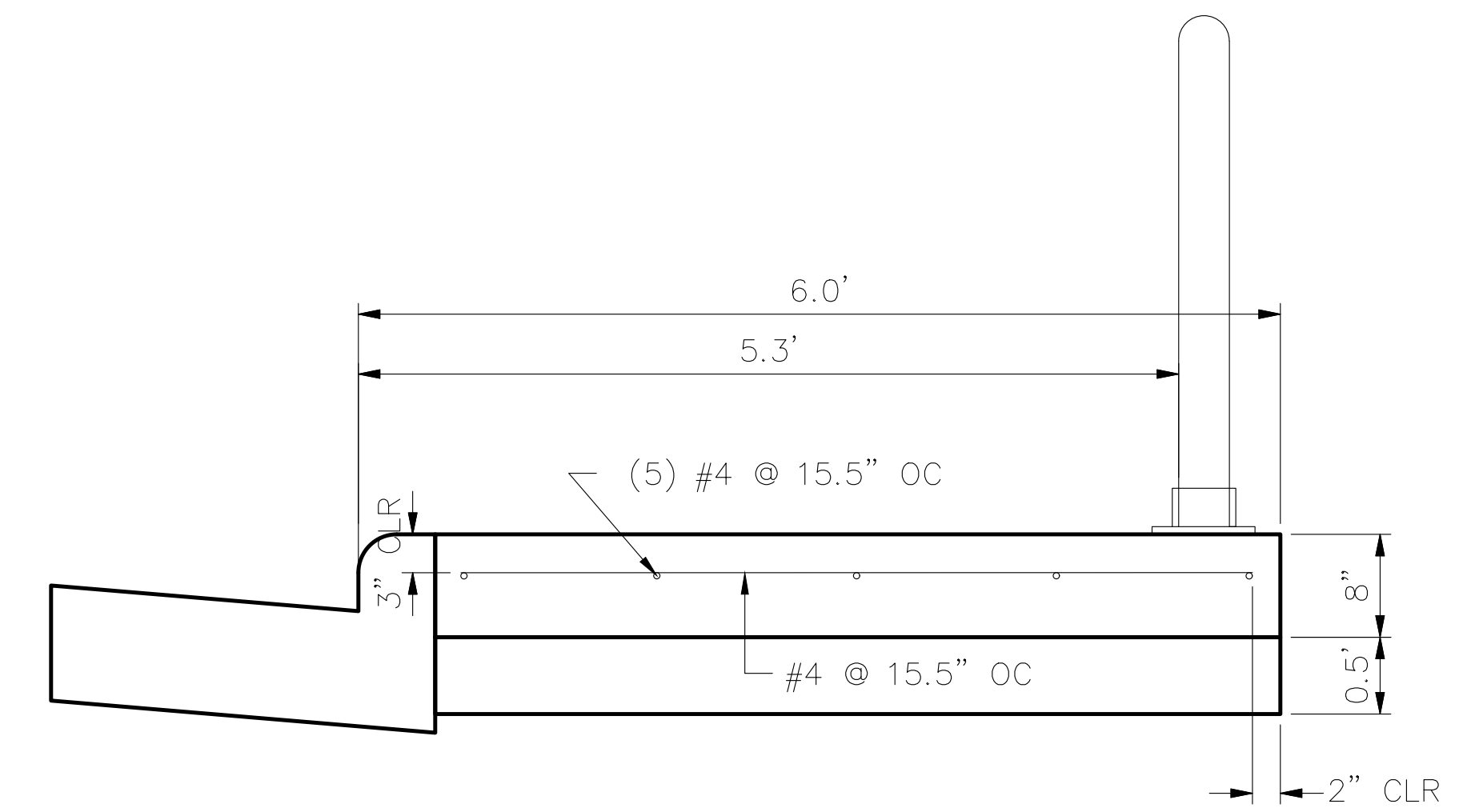
REINFORCED WALK WITH TURNDOWN CURB STA. 50+17.84 TO STA. 50+22.34
