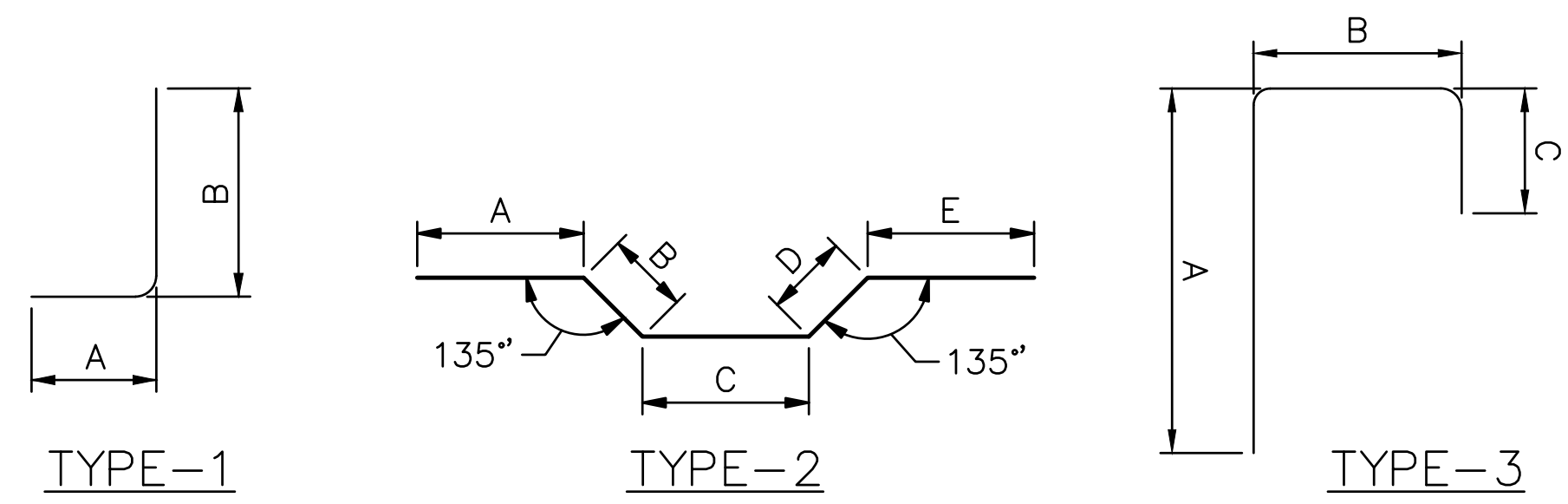
BENDING DIAGRAMS
